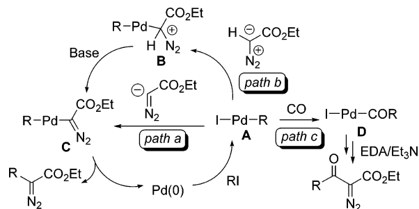
Scheme 1. Mechanistic Rationale
